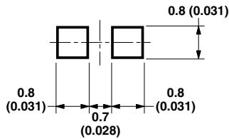
Figure 10. Recommended Soldering Pattern for HSMB-C190 and C191.
